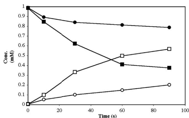
Figure 2. Exposure dependence of photo-decomposition and product formation. Compounds 3 (■) and 4 (●) are converted with greater than 90% efficiency to their parent agonist forms 1 (□) and 2 (○) but at different rates.
