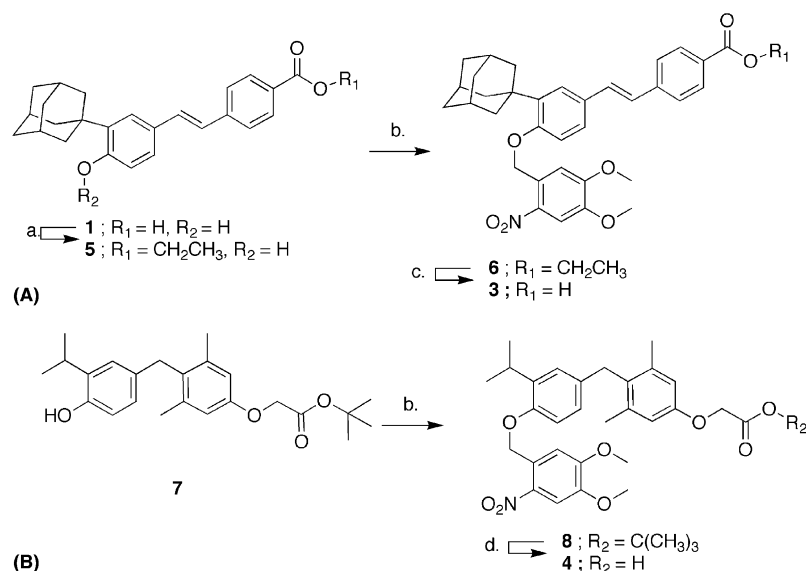
Scheme 1. Synthesis of caged agonists 3 and 4 . Reagents and conditions: (a) H_2SO_4 , EtOH, reflux (86%), (b) K_2CO_3 , nitroveratryl bromide, DMF (91%), (c) LiOH, THF/ H_2O (75%), (d) NaOH, rt (95%).
